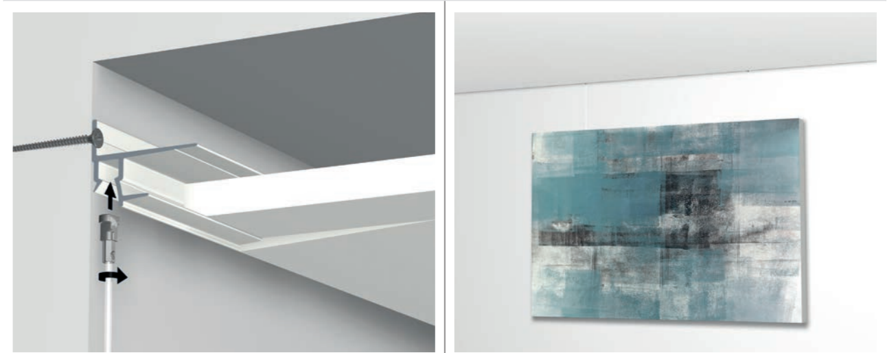
SHADOWLINE MASONRY (IN COMBINATION WITH DRYWALL)
